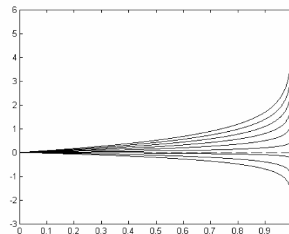
Figure 3: EVE's function for pleasure (y) versus 1-P(e), for various values of P(C|e). See text for details.
